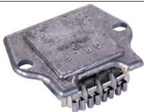
133005# Regulator 14 V, Dist. mount. holes 47.15, Terminal type G-R-L-F
