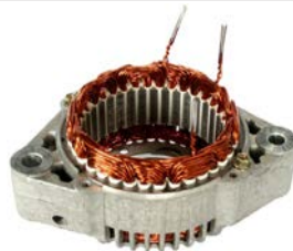
231008# Stator w/ D.E. Bracket Assy
