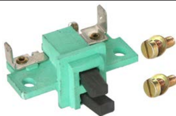
130979 Brush Box
