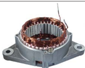
138456 Stator w/ D.E. Bracket Assy
