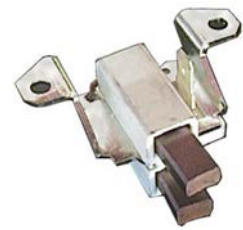
133179 Brush Box Replacing: ulb423 12 V, No./ brushes 2
