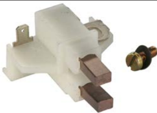
130976 Brush Box Replacing: ulb652 OD 37.50, No./ brushes 2
