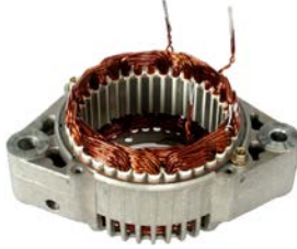
231036 Stator w/ D.E. Bracket Assy
