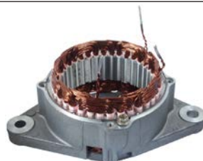
138456 Stator w/ D.E. Bracket Assy
