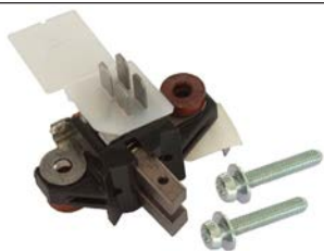
136112 Brush Box
