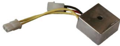
234171# Regulator/Rectifier Replacing: 691185, 397809 14 V, 8 A
