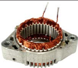
231008# Stator w/ D.E. Bracket Assy
