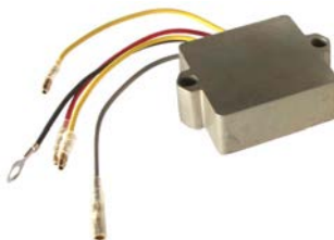
233976# Regulator/Rectifier
