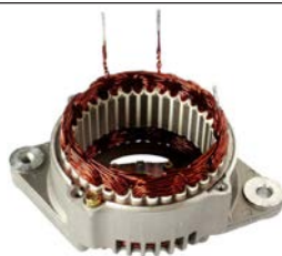
231039# Stator w/ D.E. Bracket Assy
